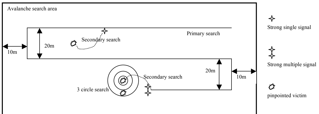
Fig. 2: The “Three Circle Method” within a multiple burial procedure is a baseline method to locate multiple victims within close range. It can be used with any beacon model.
